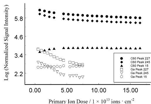
Figure 3. Normalized signal intensity as a function of C_{60}^+ or Ga^+ primary ion dose for biotin molecules on polymer resin surfaces. The peaks measured are the (M + H)^+ peak at 245.10 amu, the (M - OH)^+ peak at 227.09 amu, and the reference peak CH_3^+ at 15.02 amu.
