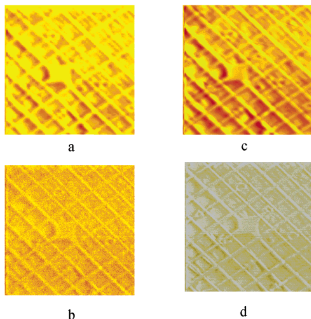
Figure 1. C_{60}^+ SEM images of 200 mesh copper grid finder on indium foil obtained with various energies and beam apertures: (a) at 10 keV beam energy and 100 \mu\text{m} beam aperture; (b) at 10 keV beam energy and 30 \mu\text{m} beam aperture; (c) at 20 keV beam energy and 100 \mu\text{m} beam aperture; (d) at 20 keV beam energy and 30 \mu\text{m} beam aperture. All images are 1000 \mu\text{m} \times 1000 \mu\text{m} .
