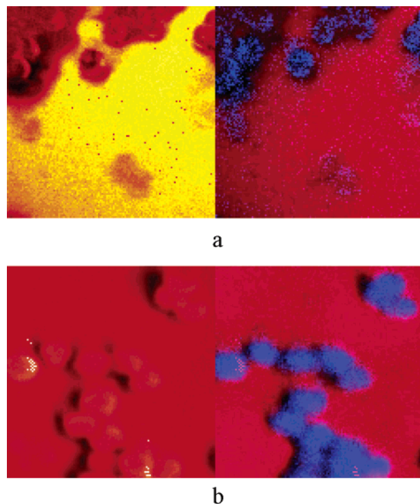
Figure 2. SIMS images of Biotin-Sasrin linker–copoly (styrene–1% DVB) resins acquired with \text{Ga}^+ (a) and \text{C}_{60}^+ (b), respectively. The resins are placed on silicon substrate and are examined after biotin molecules are released from the Sasrin linker by vapor-phase TFA. In both panels, the images on the left are total ion images. For the images on the right, the molecular ions of biotin are pictured in blue and silicon substrate ions are pictured in red. Image size: 400 \mu\text{m} \times 400 \mu\text{m} .
