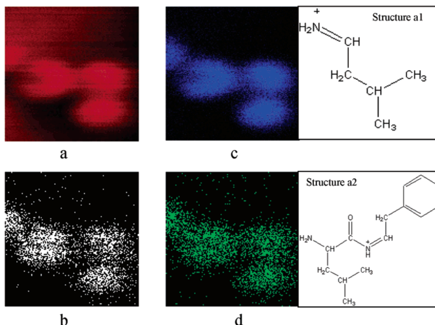
Figure 7. SIMS images of Leu-(Phe) 3 -Rink Amide MBHA resins measured with C 60 + . (a) Total ion image. (b) Molecular ion image. (c) Image of fragmentation peak at m/z 86.10, which corresponds to structure a1. (d) Image of fragmentation peak at m/z 233.17, which corresponds to structure a2. Image size is 450 \mu m \times 450 \mu m.
